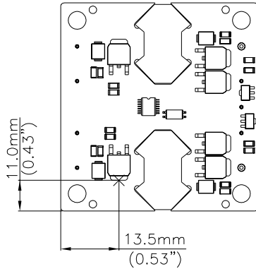
Figure 20: Temperature measurement location * The allowed maximum hot spot temperature is defined at 123 °C
