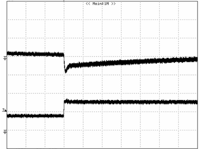
Figure 9: Output voltage response to step-change in load current (25%-50% of I_o , max; di/dt = 0.1A/\mu s ). Load cap: 47\mu F aluminum capacitor and 1\mu F ceramic capacitor. TOP Trace: V_{out} (1V/div), Bottom Trace: I_{out} (1A/div), Scope measurement should be made using a BNC cable (length shorter than 20 inches). Position the load between 51 mm to 76 mm (2 inches to 3 inches) from the module.
