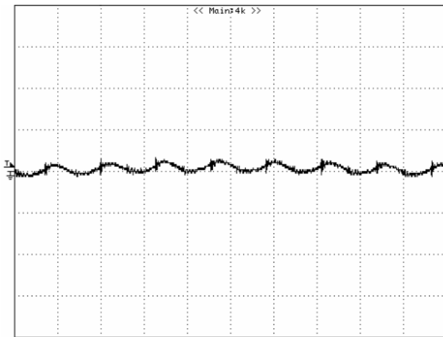
Figure 12: Input reflected ripple current, i_s , through a 12\mu\text{H} source inductor at nominal input voltage and rated load current ( 20\text{mA/div} , 2\text{us/div} ).
