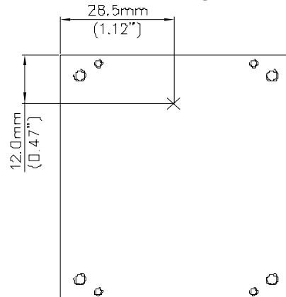
Figure 22: Temperature measurement location * The allowed maximum hot spot temperature is defined at 100 °C
