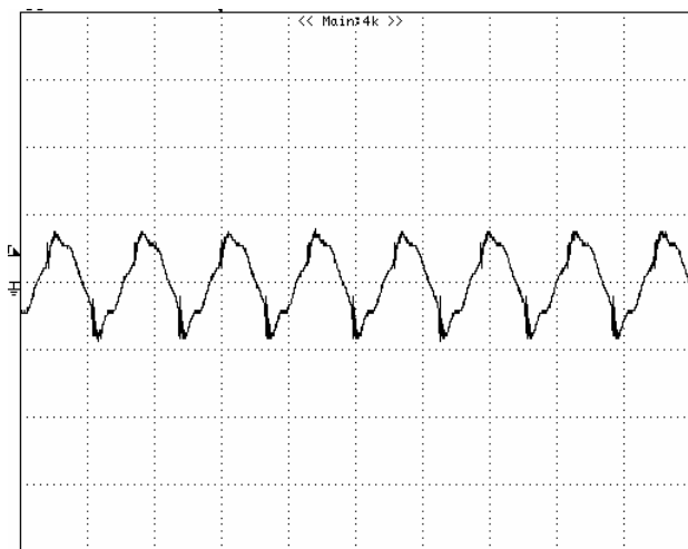
Figure 14: Output voltage ripple at nominal input voltage and rated load current ( I_o=3.2\text{A} ) ( 50\text{mV/div} , 2\text{us/div} ). Load capacitance: 1\mu\text{F} ceramic capacitor and 470\mu\text{F} electrolytic capacitor. Bandwidth: 20\text{MHz} . Scope measurements should be made using a BNC cable (length shorter than 20 inches). Position the load between 51 mm to 76 mm (2 inches to 3 inches) from the module.
