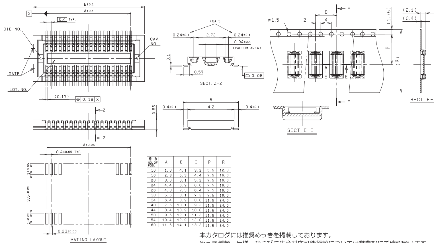
MOUNTING LAYOUT
