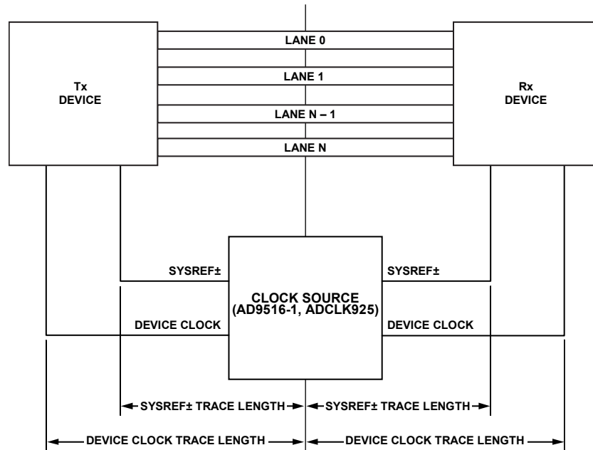
Figure 83. SYSREF \pm Signal and Device Clock Trace Length
