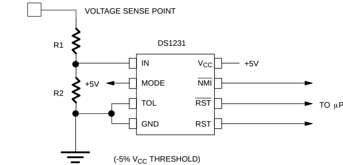
APPLICATION WITH MODE PIN CONNECTED TO V CC Figure 4
