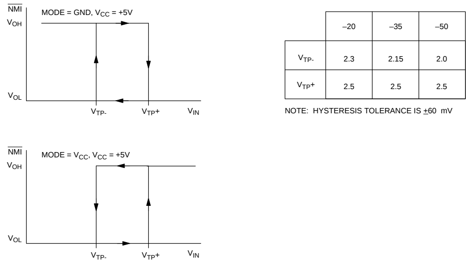
INPUT PIN HYSTERESIS Figure 3
