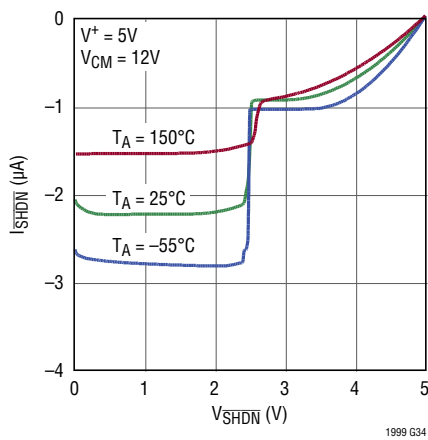
SHDN Pin Current vs SHDN Pin Voltage and Temperature
