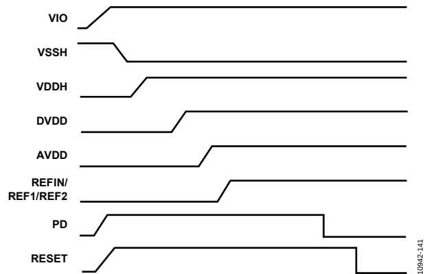
Figure 46. Power-Up Sequence
