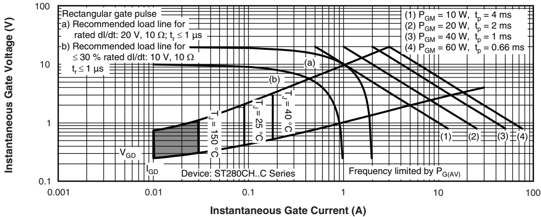
Fig. 11 - Gate Characteristics
