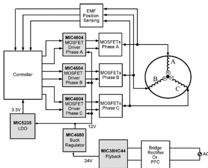
Figure 12. 3-Phase Brushless DC Motor Driver – 24V Block Diagram
