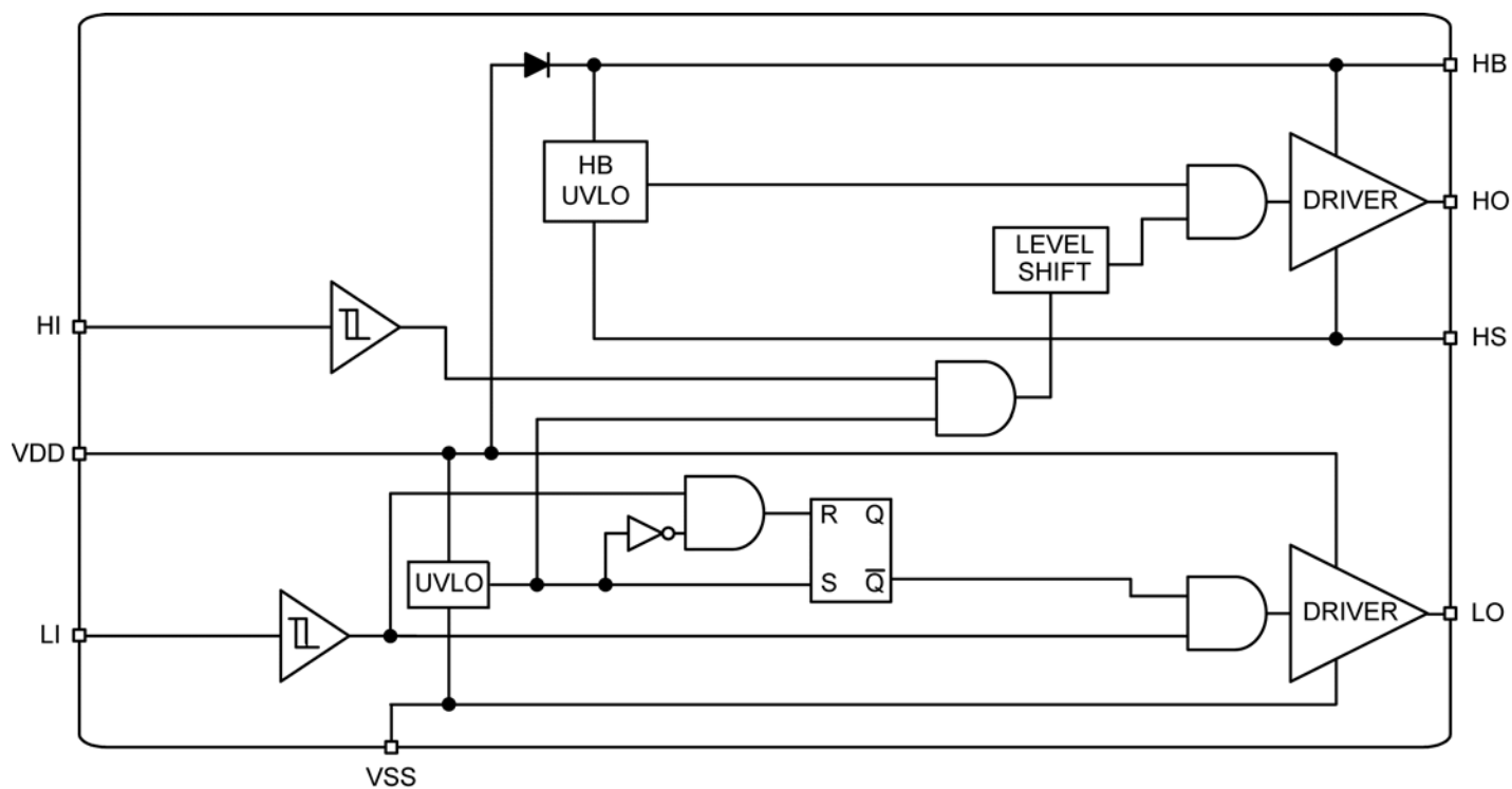
Figure 1. MIC4604 Block Diagram
