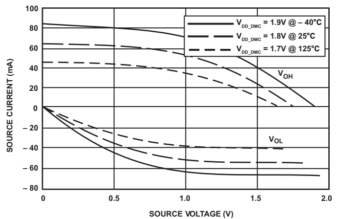
Figure 57. Driver Type C Current ( 1.8\text{ V } V_{DD\_DMC} )
