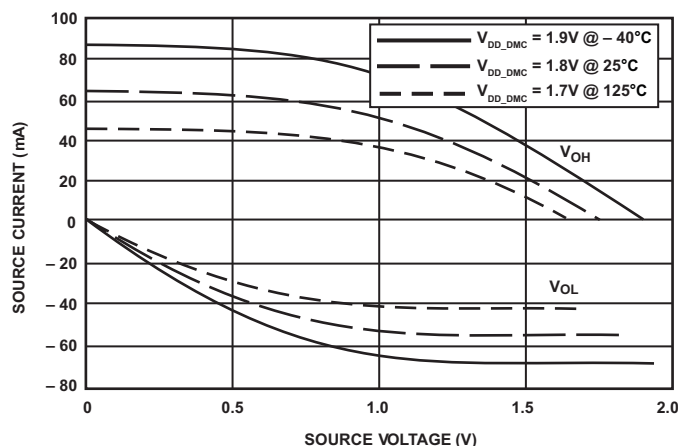
Figure 56. Driver Type B Current ( 1.8\text{ V } V_{DD\_DMC} )
