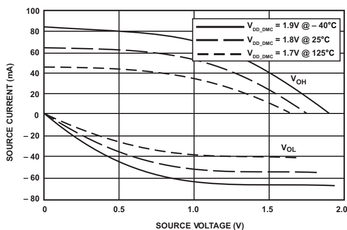
Figure 57. Driver Type C Current ( 1.8\text{ V } V_{DD\_DMC} )
