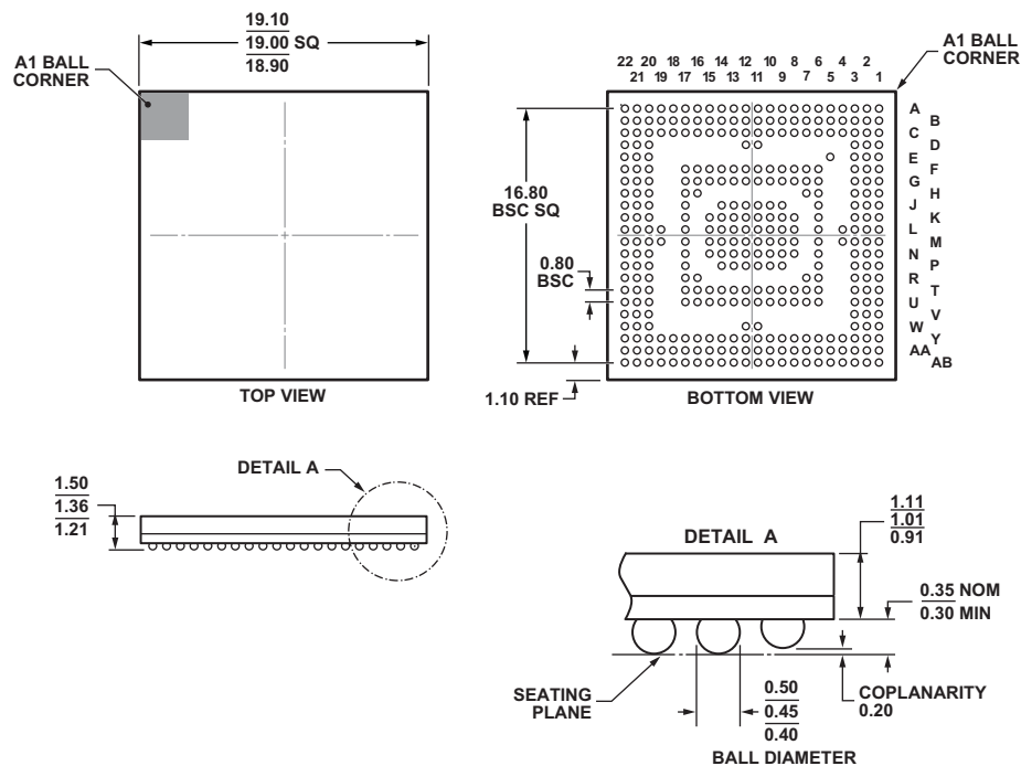
COMPLIANT TO JEDEC STANDARDS MO-275-PPAB-2. Figure 65. 349-Ball Chip Scale Package Ball Grid Array [CSP_BGA] (BC-349-1) Dimensions shown in millimeters
