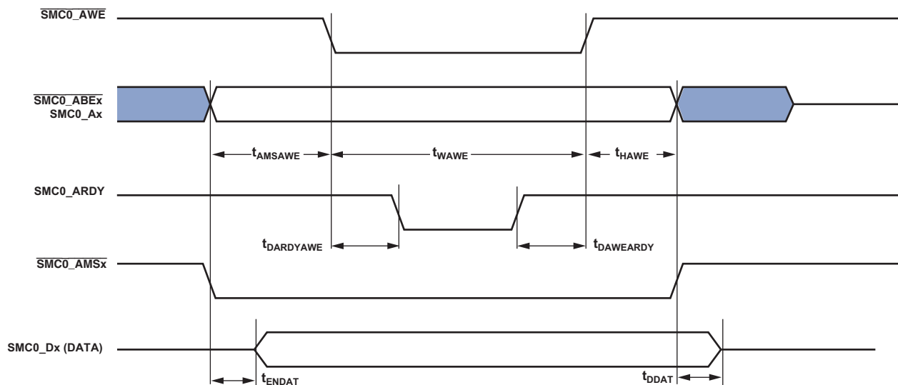
Figure 16. Asynchronous Write
