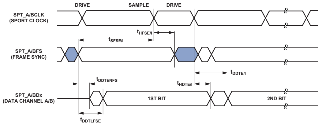
Figure 34. External Late Frame Sync
