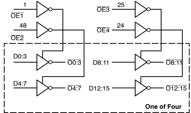
Figure 2. Logic Diagram
