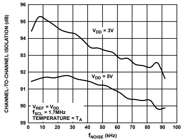
Figure 14. AD7991 Channel-to-Channel Isolation, f_{SCL} = 1.7MHz Without Clock Stretching
