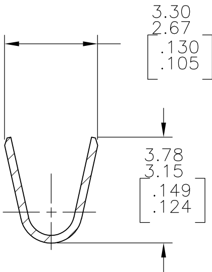
SECTION B-B
