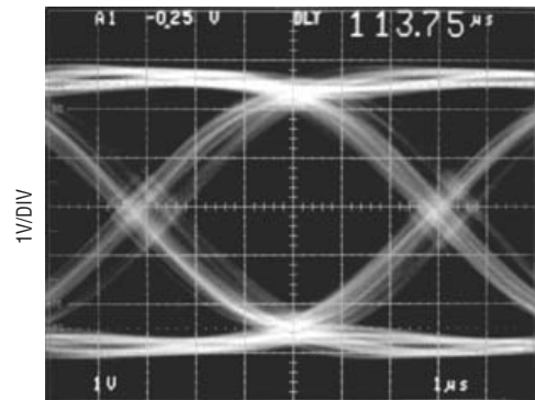
Eye Diagram
