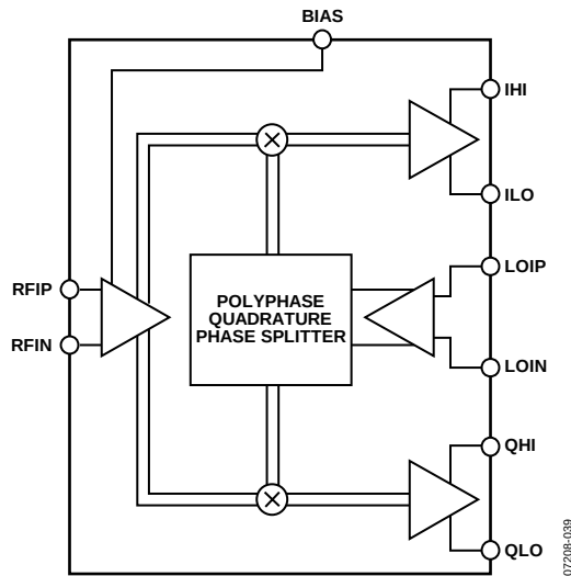
Figure 39. Block Diagram
