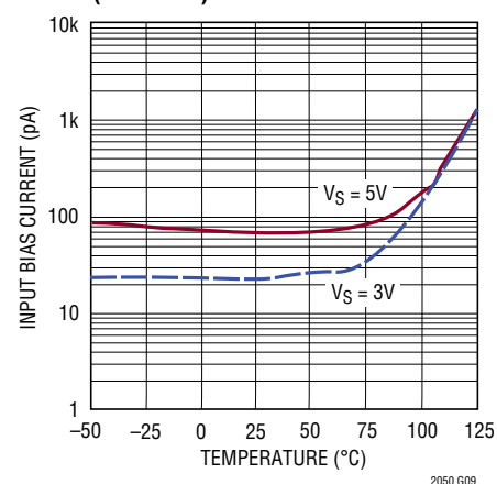
Input Bias Current vs Temperature (LTC2050)
