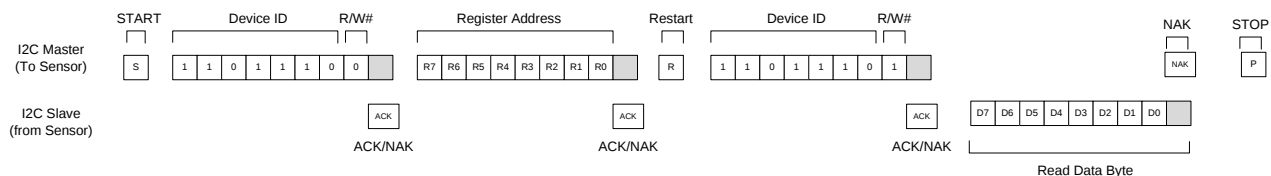
Figure 9. I2C Message Format, Read Cycle, Single Register Read
