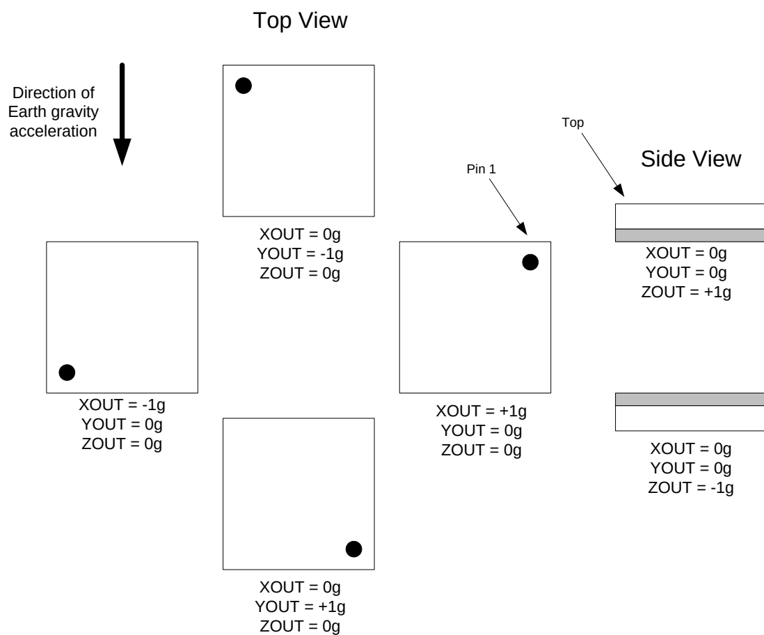
Figure 3. Package Orientation
