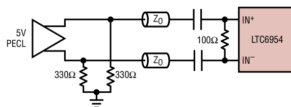
AC-COUPLED 5V PECL
