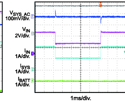
System Current Transient Battery Full, I_{SYS} = 1-2A transient, 0.05A/µs
