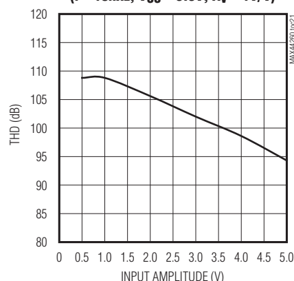
TOTAL HARMONIC DISTORTION vs. INPUT AMPLITUDE ( f = 10kHz , V_{CC} = 5.5V , A_V = 1V/V )
