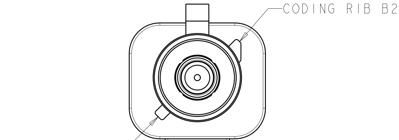
DETAIL I
