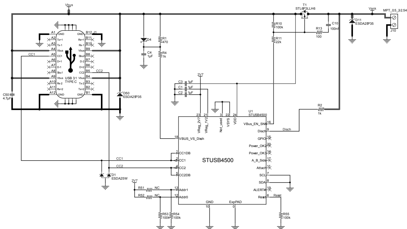
Figure 9. STUSB4500 schematic
