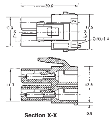
Section X-X
