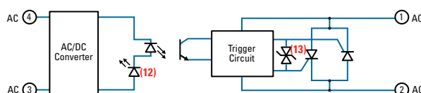
Diagram: HA60xxT
