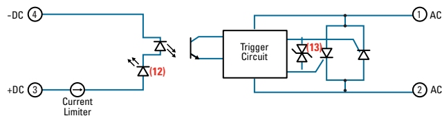
Diagram: HD60xxxxT
