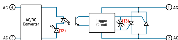
Diagram: HA60xxT
