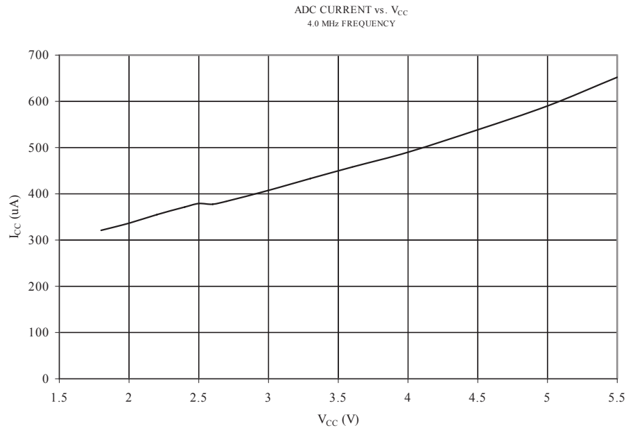
Figure 18-46. ADC Current vs. V_{CC} (ATtiny5/10, only)
