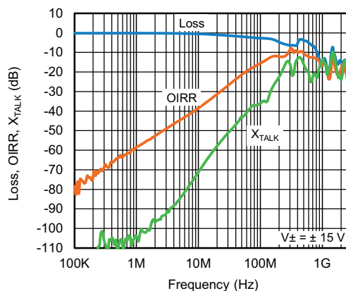
BW, OIRR, X_{TALK} vs. Frequency
