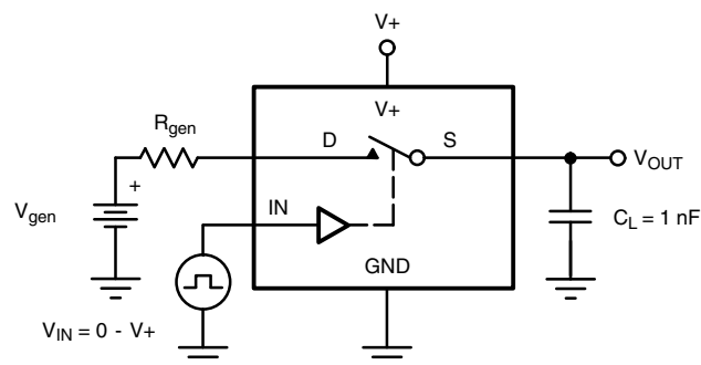
Fig. 2 - Charge Injection
