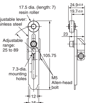
WL-2A111 Resin Roller
