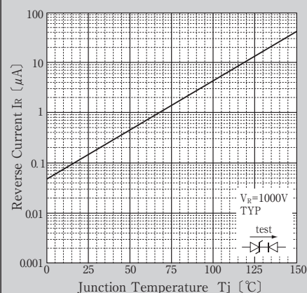
逆電流 - 接合部温度 Reverse Current vs Junction Temperature
