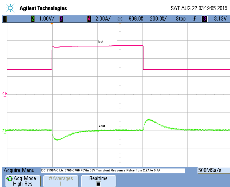
Figure 4. Transient Response Waveform at 48V IN and 2.7A to 5.4A to 2.7A OUT (2A, 1V, 200μs/DIV)
