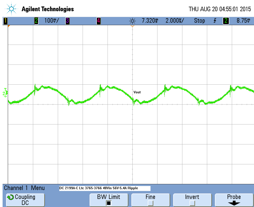
Figure 3. Output Ripple at 48V IN and 5.4A OUT (100mV, 2μs/DIV, 20MHz)
