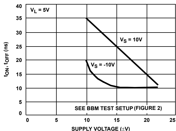
FIGURE 23. BREAK-BEFORE-MAKE vs POWER SUPPLY VOLTAGE
