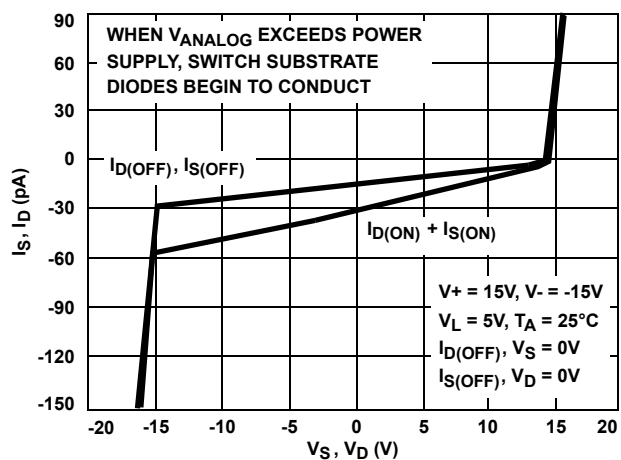
FIGURE 20. LEAKAGE CURRENTS vs ANALOG VOLTAGE
