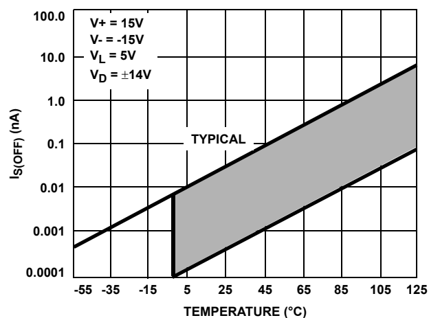
FIGURE 17. I_{S(OFF)} vs TEMPERATURE
