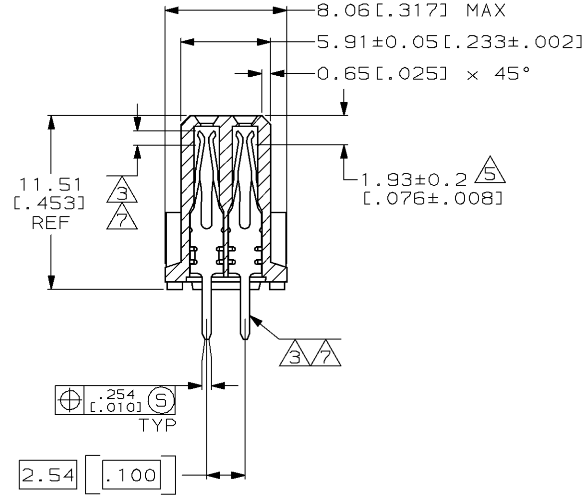
SECTION X-X
