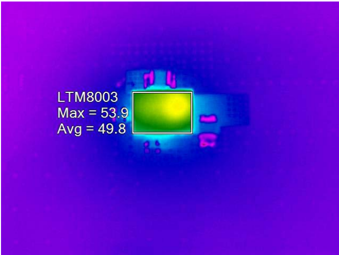
(4a) V_{IN} = 12V
