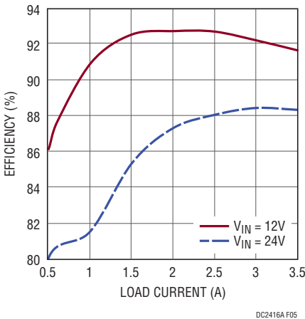
Figure 5. DC2416A Efficiency vs Load Current ( T_A = 25^\circ C )
