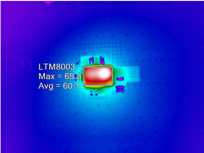
(4b) V_{IN} = 24V
