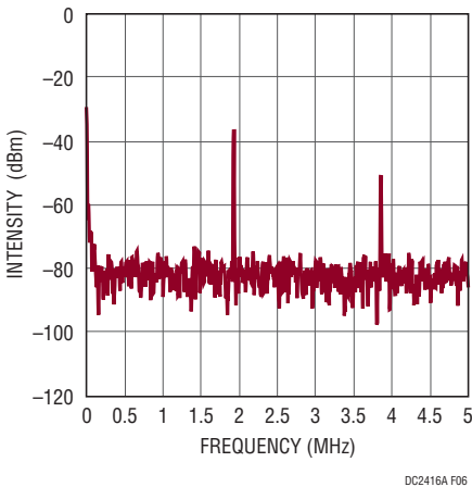
Figure 6. Output Noise Spectrum with 3.5A Load Current ( V_{IN} = 12V )
