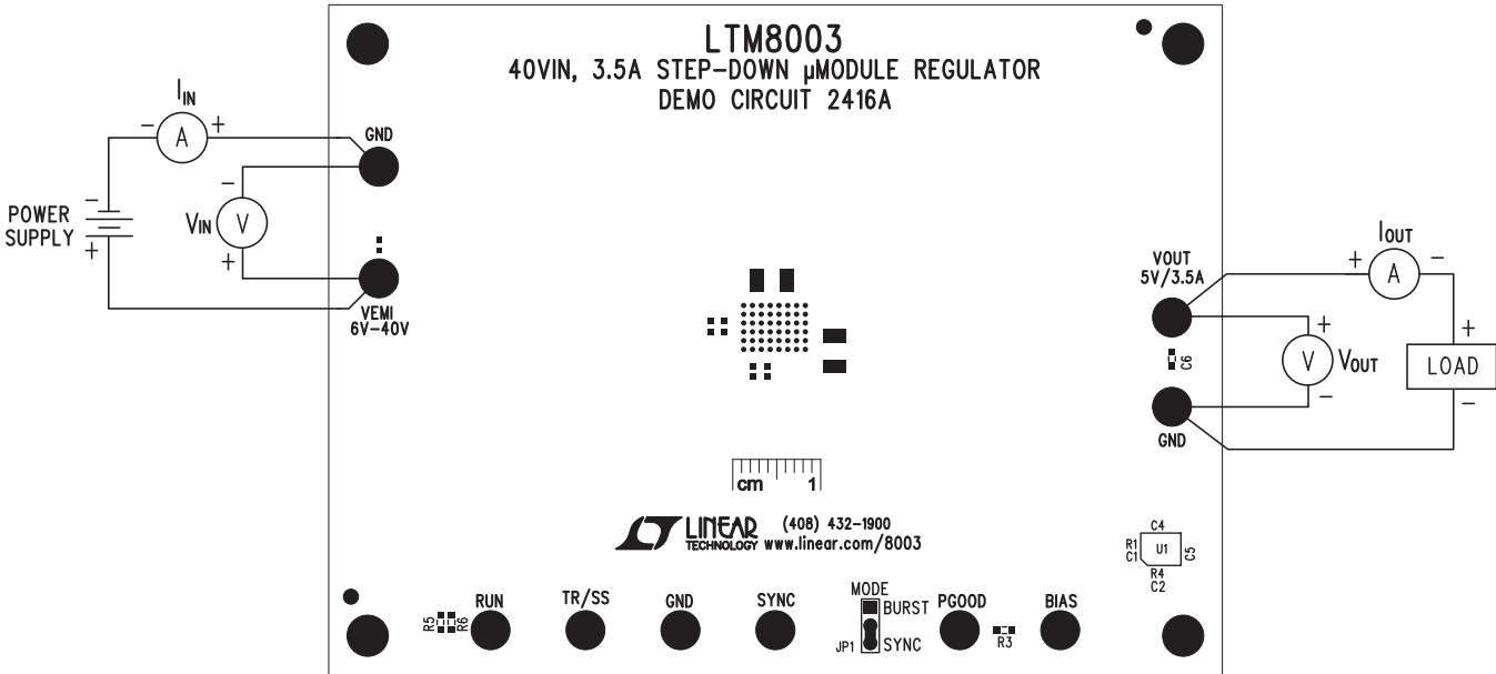
Figure 1. DC2416A Proper Equipment Setup
