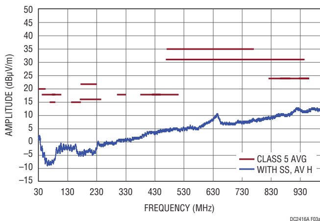
(3a) Horizontal Polarization, Average, with Spread Spectrum
