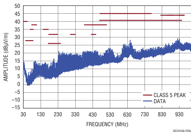
(3d) Vertical Polarization, Peak, without Spread Spectrum
