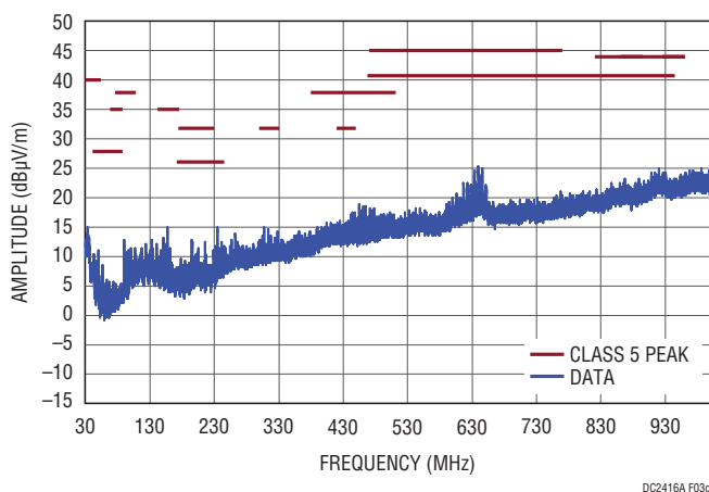
(3c) Horizontal Polarization, Peak, without Spread Spectrum
