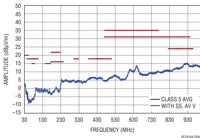
(3b) Vertical Polarization, Average, with Spread Spectrum
