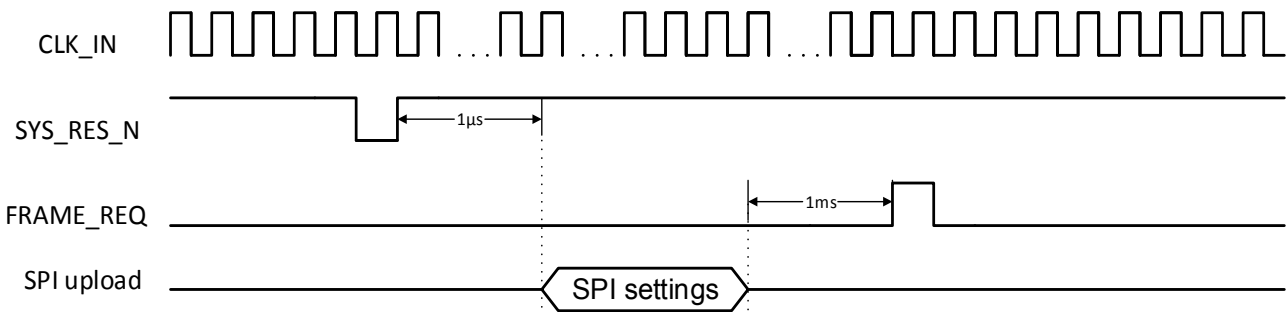
Figure 10: Reset sequence when changing bit mode
