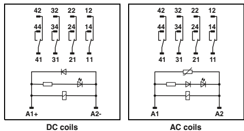
DC coils
