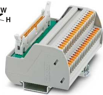
Passive interface modules for input/output, with specific marking and push-in connection
