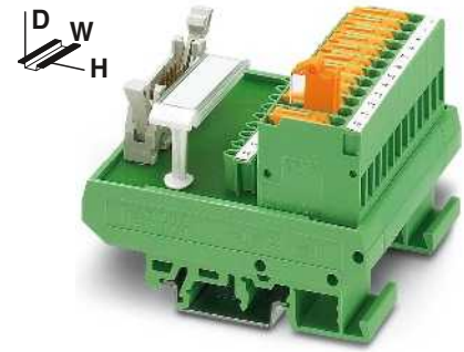
Passive interface modules for eight or 32 channels with knife disconnect terminal blocks
