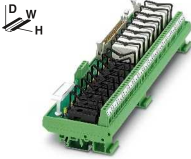
Output base module with 16 miniature relays, 1 PDT
