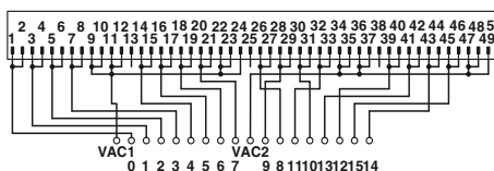
Connection scheme VIP-2/.../FLK50/16/SLC500
