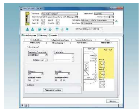
Relay configuration
