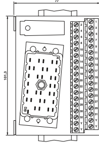
Dimensional drawing for UMK-EC90/32/EX-XUL
