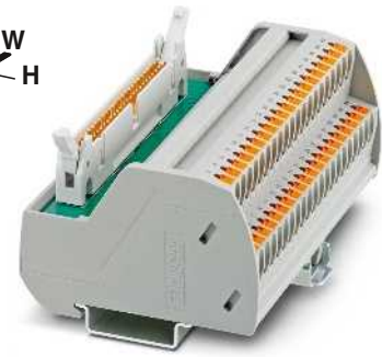
Passive interface modules for input/output, with specific marking and push-in connection
