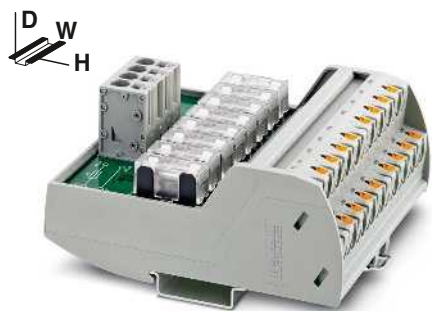
With push-in connection and 2 potential levels and eight 6.3 A fuses
