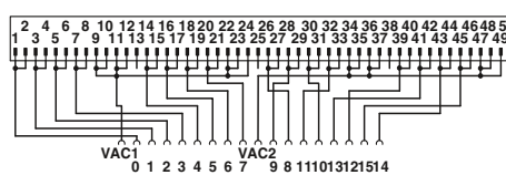
Connection scheme FLKM 50-PA-SLC500/OUT/2A
