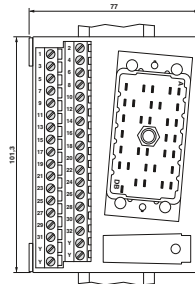
Dimensional drawing for UMK-EC90/32/EX-XOR
