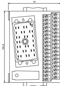
Dimensional drawing for UMK-EC90/32/EX-XOL
