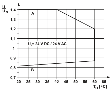
Permissible input voltage range for PLC-RS...24UC/1/S...
