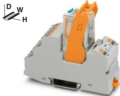
RIF-2 relay module with 4 PDT relay
