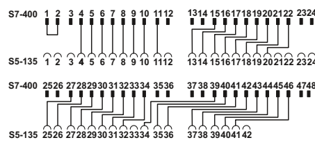
FLKM S135-431-UA/S400 connection scheme
