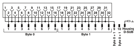
FLKM-PA-2D15/HW/DI/C300 connection scheme
