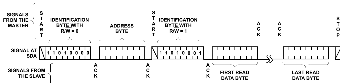
FIGURE 11. READ SEQUENCE
