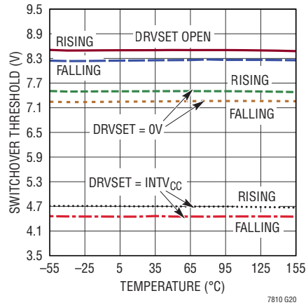
EXT CC Switchover Thresholds vs Temperature
