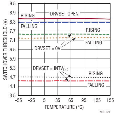
EXT VC Switchover Thresholds vs Temperature
