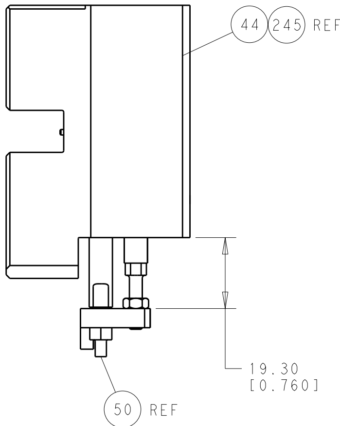
HOLDDOWN SET-UP
