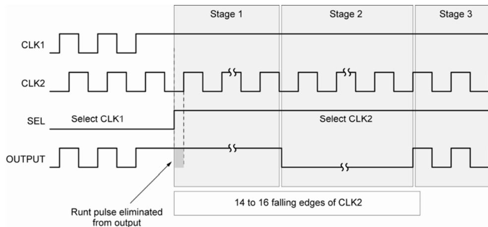
Timing Diagram 2
