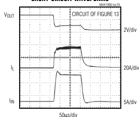
MAX1960/MAX1961 SHORT-CIRCUIT WAVEFORMS
