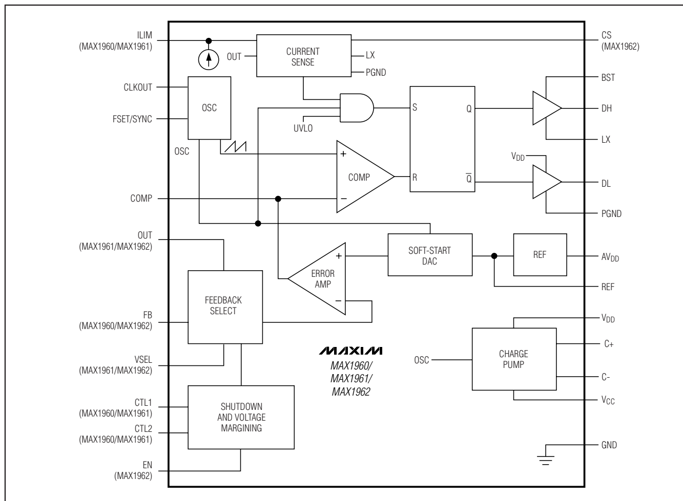
Figure 1. Functional Diagram
