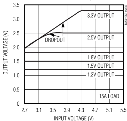
OUTPUT VOLTAGE vs. INPUT VOLTAGE, 1MHz
