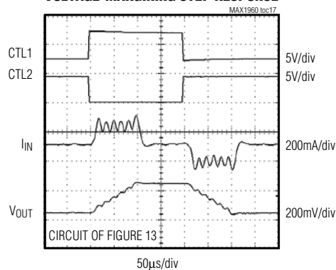
VOLTAGE-MARGINING STEP RESPONSE
