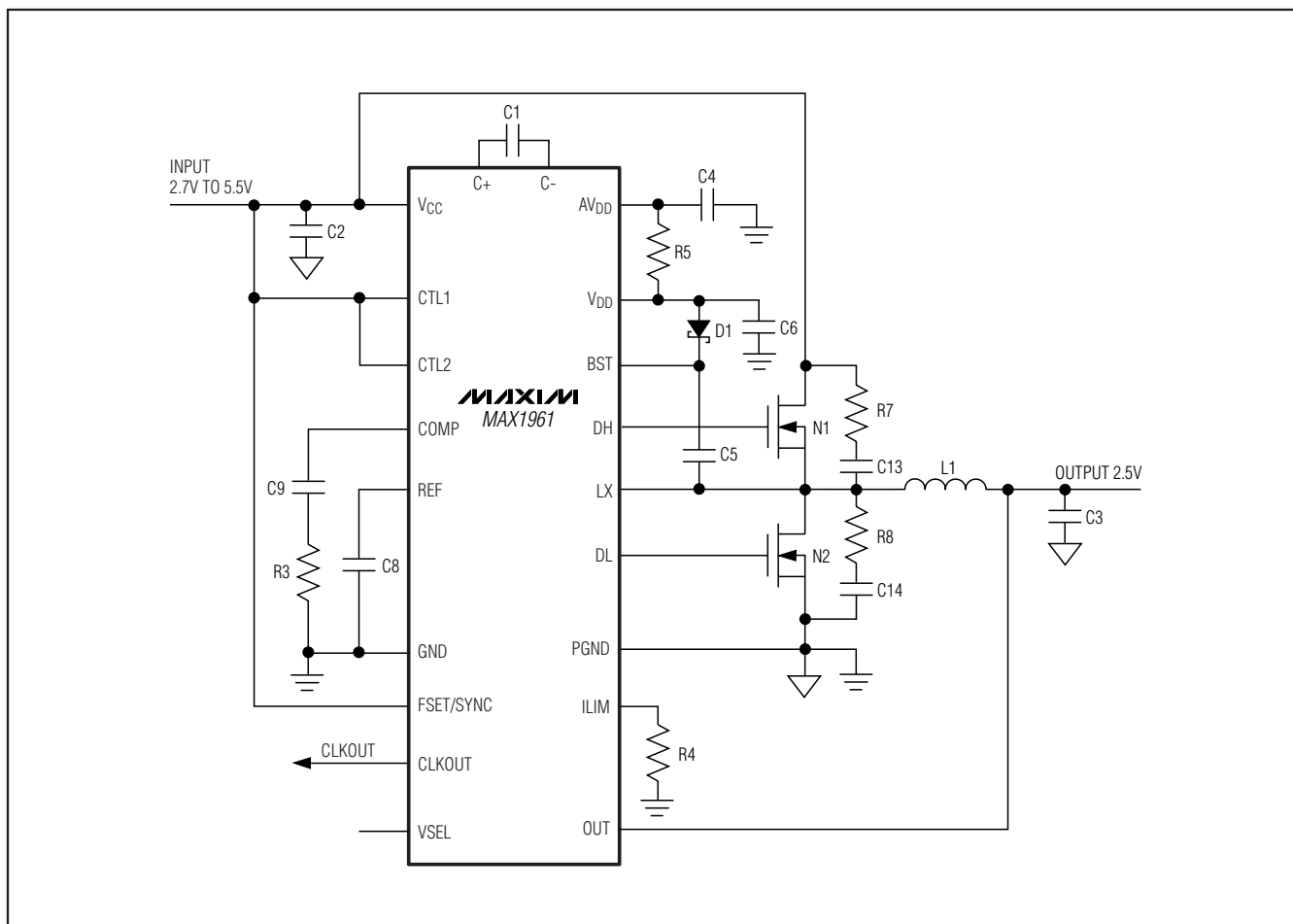
Figure 10. Application Circuit 2—MAX1961 Preset Output Voltage
