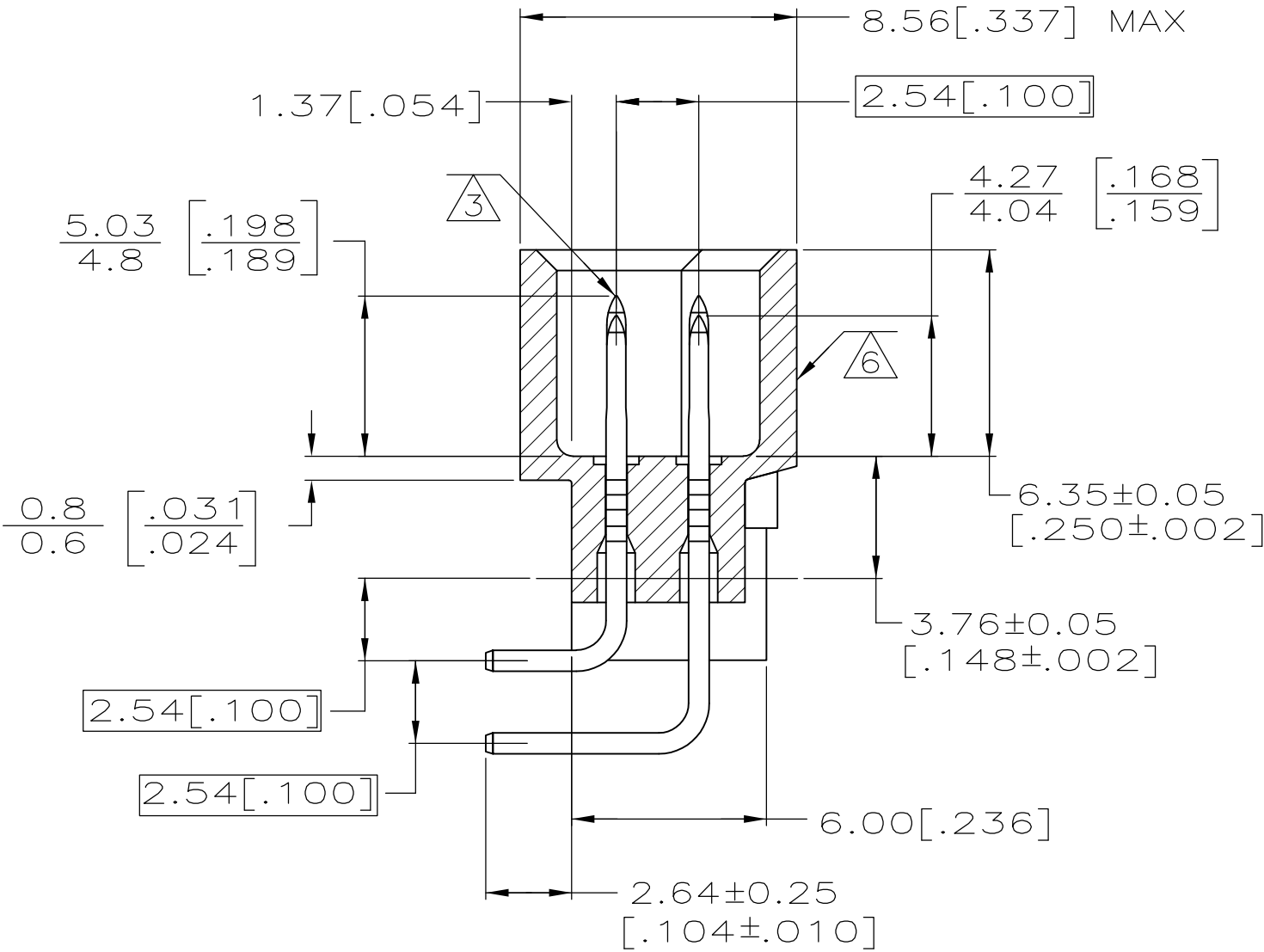
SECTION X-X
