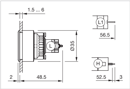
Dimensions [mm] L = Solder terminal, L1 = Solder terminal 2.8 x 0.5 mm, H = Universal terminal 2.0 x 0.5 mm
