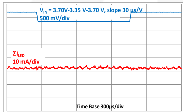
Figure 12. Line Transient Response V_{IN} = 3.70\text{ V} - 3.35\text{ V} - 3.70\text{ V} with I_{LED} = 5 \times 25\text{ mA}
