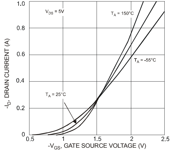
Fig. 12 Typical Transfer Characteristics
