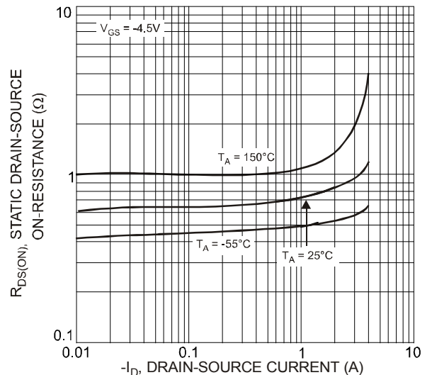
Fig. 14 Static Drain-Source On-Resistance vs. Drain Current
