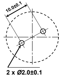
PC Board Mounting Holes
