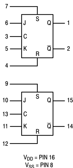
BLOCK DIAGRAM
